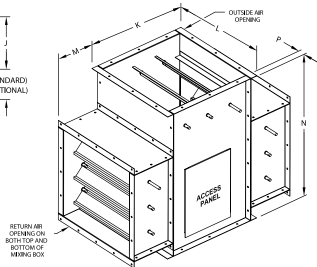
MIXING BOX
