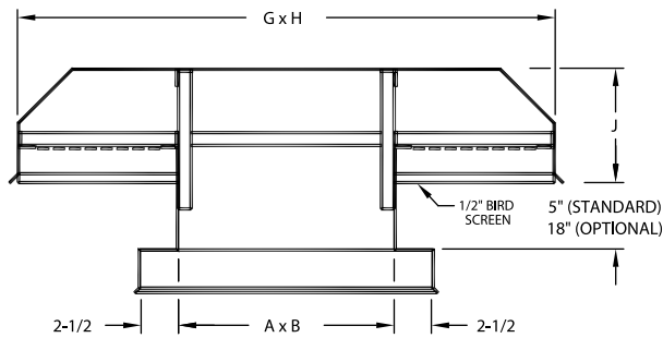
INTAKE HOOD
