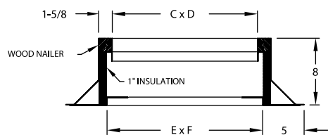
FLAT ROOF CURB SECTION
